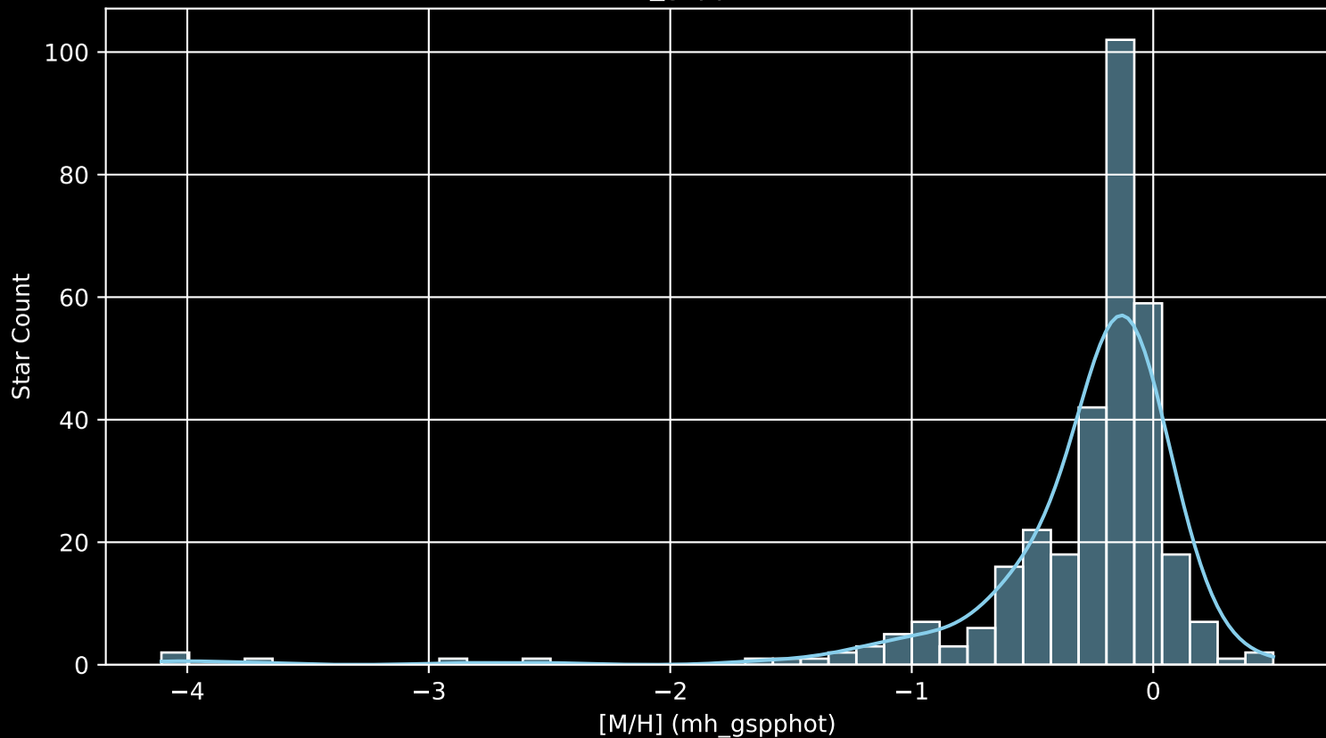
APOGEE DR17 Field: [LAMBDAORI-C [M/H] (mh_gspphot) (n= 321)
