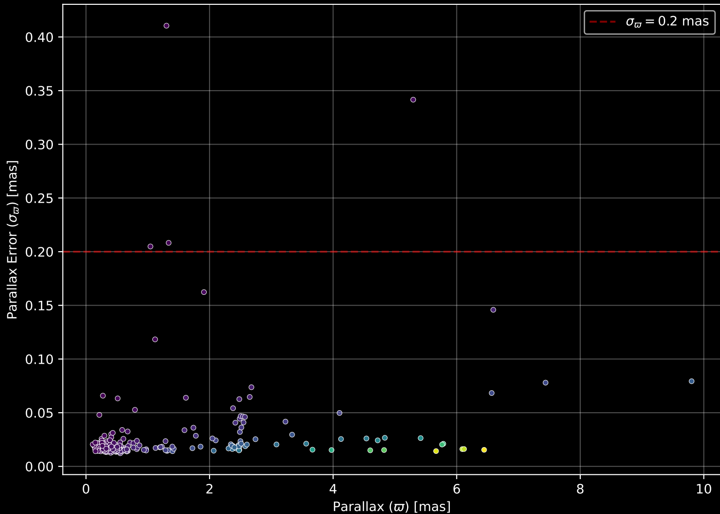
APOGEE DR17 Field: [LAMBDAORI-C] Parallax Quality (n= 324)
