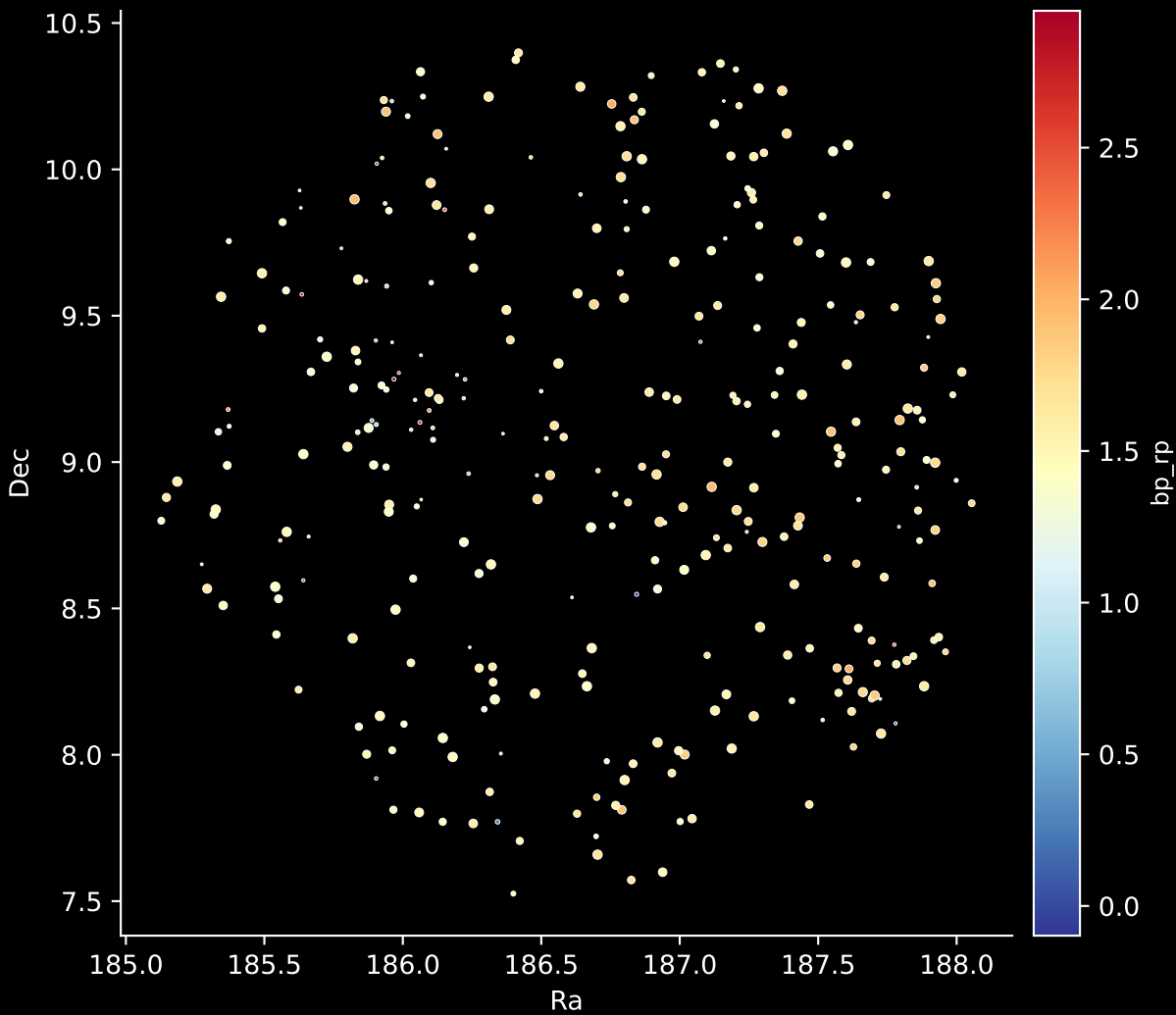
APOGEE DR17 Field: [LAMBDAORI-C] Stars: 324
