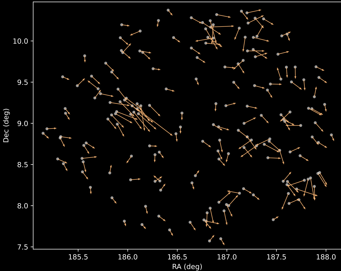
APOGEE DR17 Cluster 3 Proper Motion Vectors (n=180)
