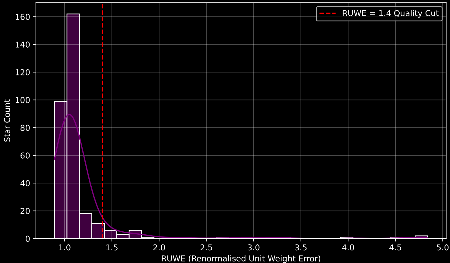
GAPOGEE DR17 Field [LAMBDAORI-C] RUWE Distribution (n= 316)
