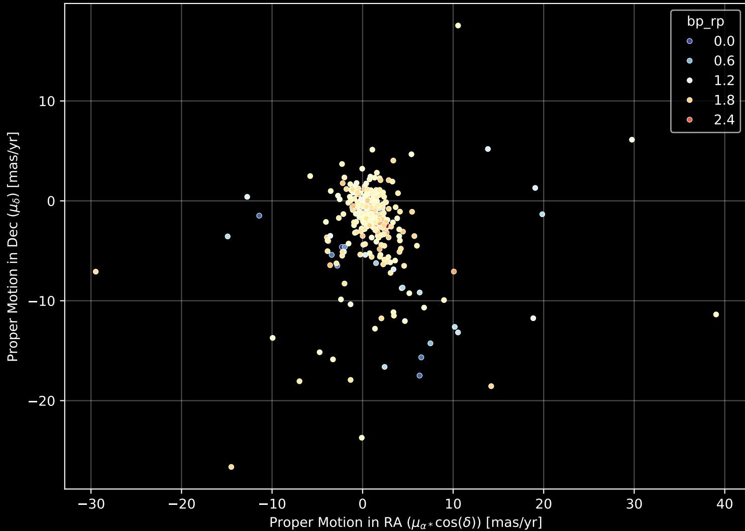
APOGEE DR17 Field: [LAMBDAORI-C] Proper Motion Diagram (n= 324)
