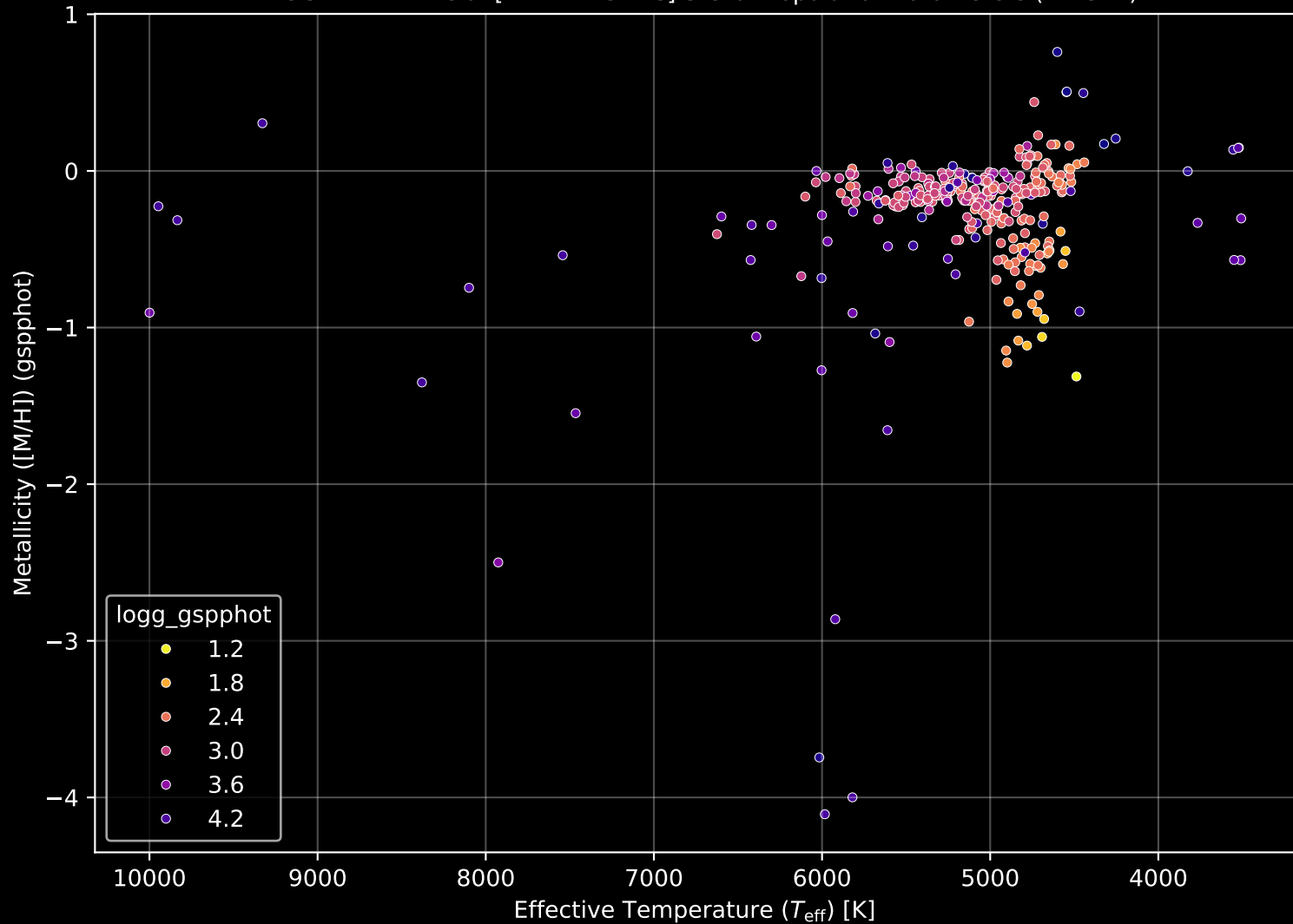
APOGEE DR17 Field: [LAMBDAORI-C] Stellar Population Parameters (n= 324)
