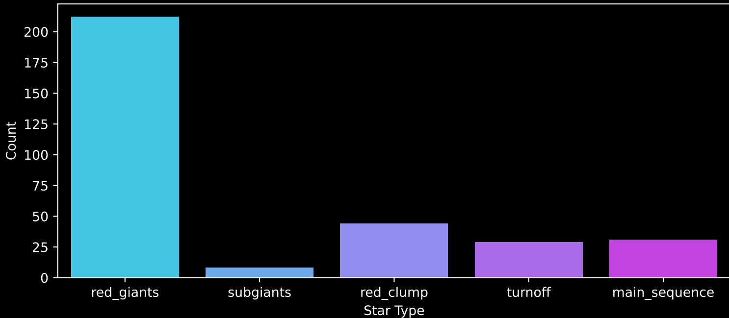
APOGEE DR17 Field: [LAMBDAORI-C] Count plot of Star Type
